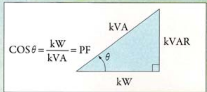
Figure 1: Power Triangle :
